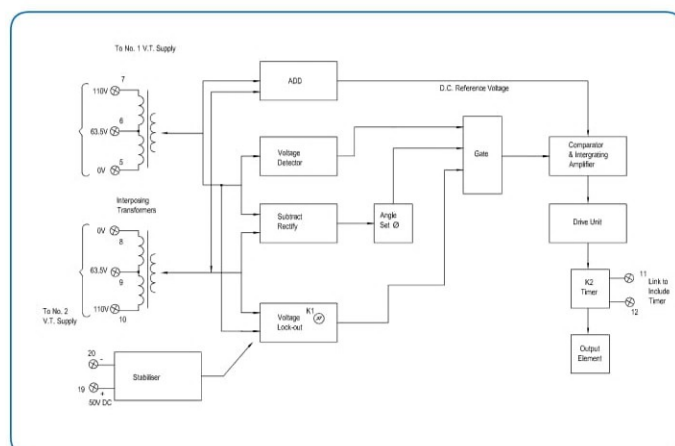
Figure 2: Composite block diagram
