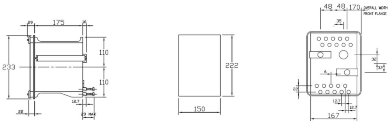
Figure 3 : Case and panel cut-out dimensions for case 1D ( All dimensions in mm)
